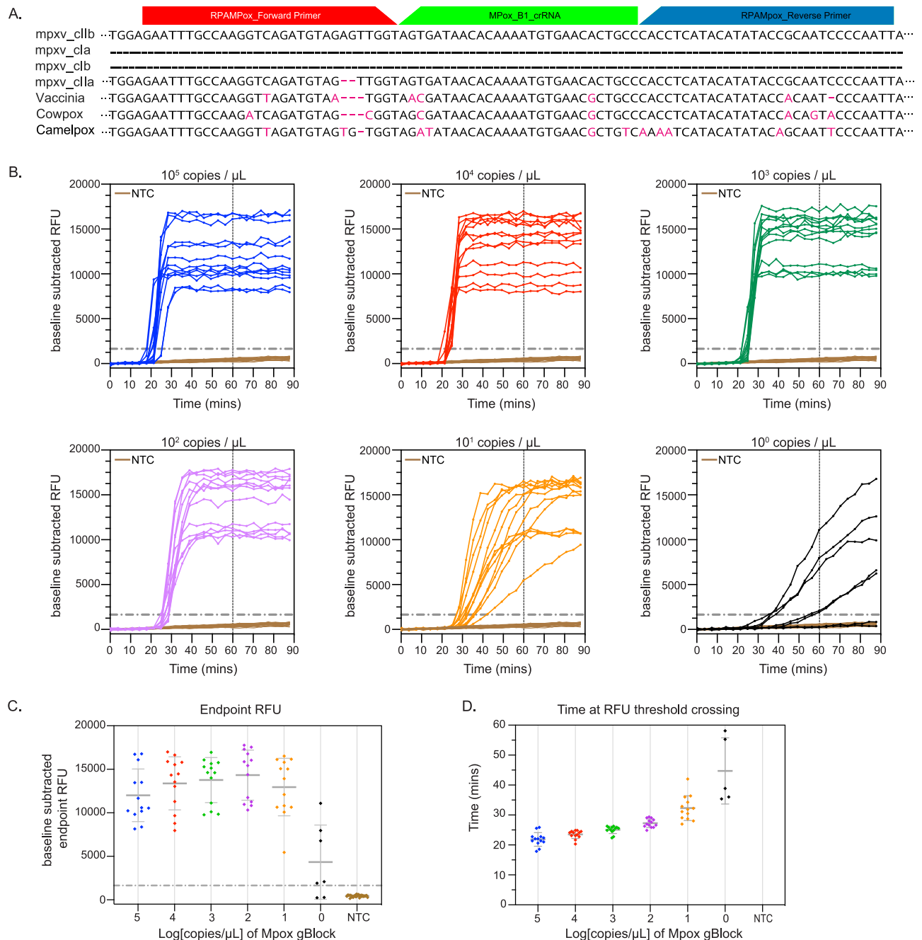
Fig. 1 | Mpx SHINE assay design and analytical performance on a plate reader.
